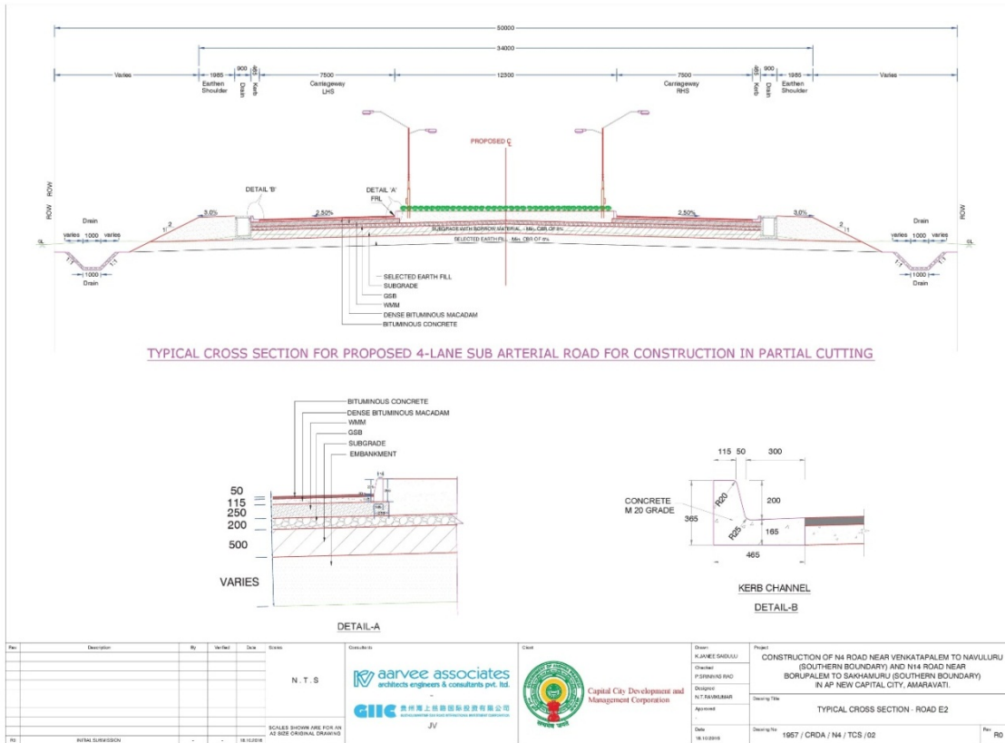
Figure 2-8: TCS for proposed 4-Lane Sub-arterial road for construction in Partial Cutting
