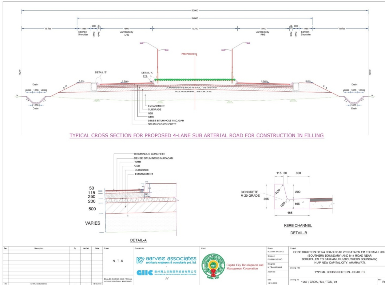
Figure 2-7: TCS for proposed 4-Lane Sub-arterial road for construction in Filling
